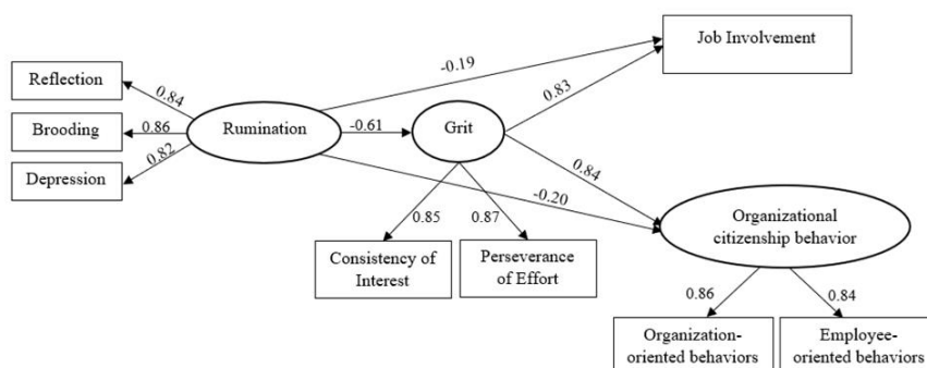
Figure 2. Standardized regression weights for the final model paths
